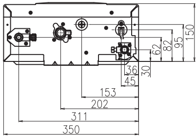
GQ-11D2AFE (X) 底面图示
