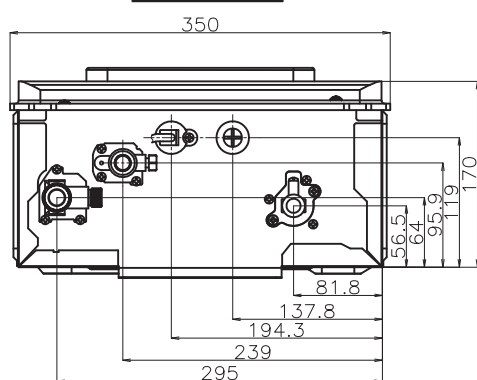
GQ-20D2AW底面图
